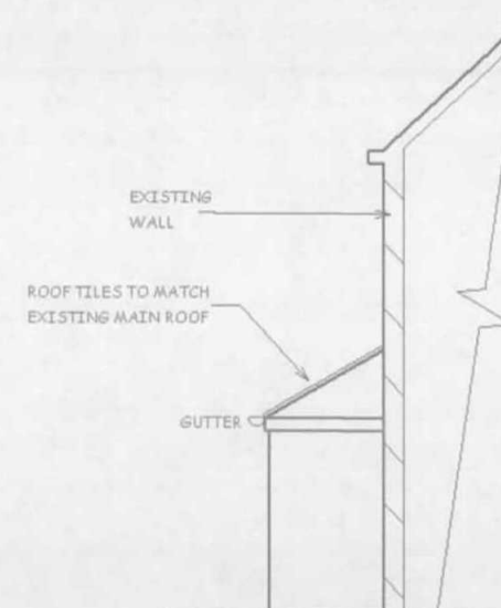
PROPOSED RIGHT HAND ELEVATION
