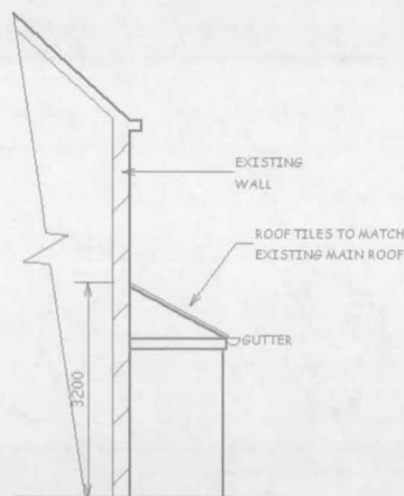
PROPOSED LEFT HAND ELEVATION
