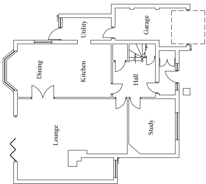
EXISTING GROUND FLOOR LAYOUT
