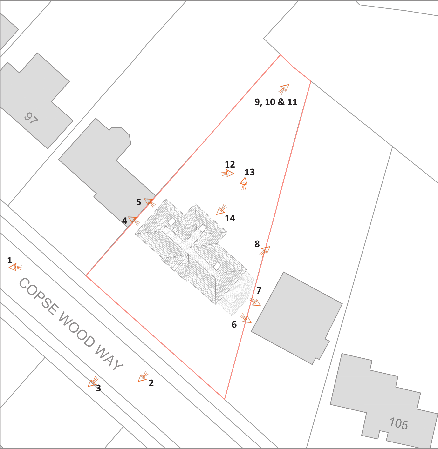
EXISTING SITE PLAN: IMAGE KEY
