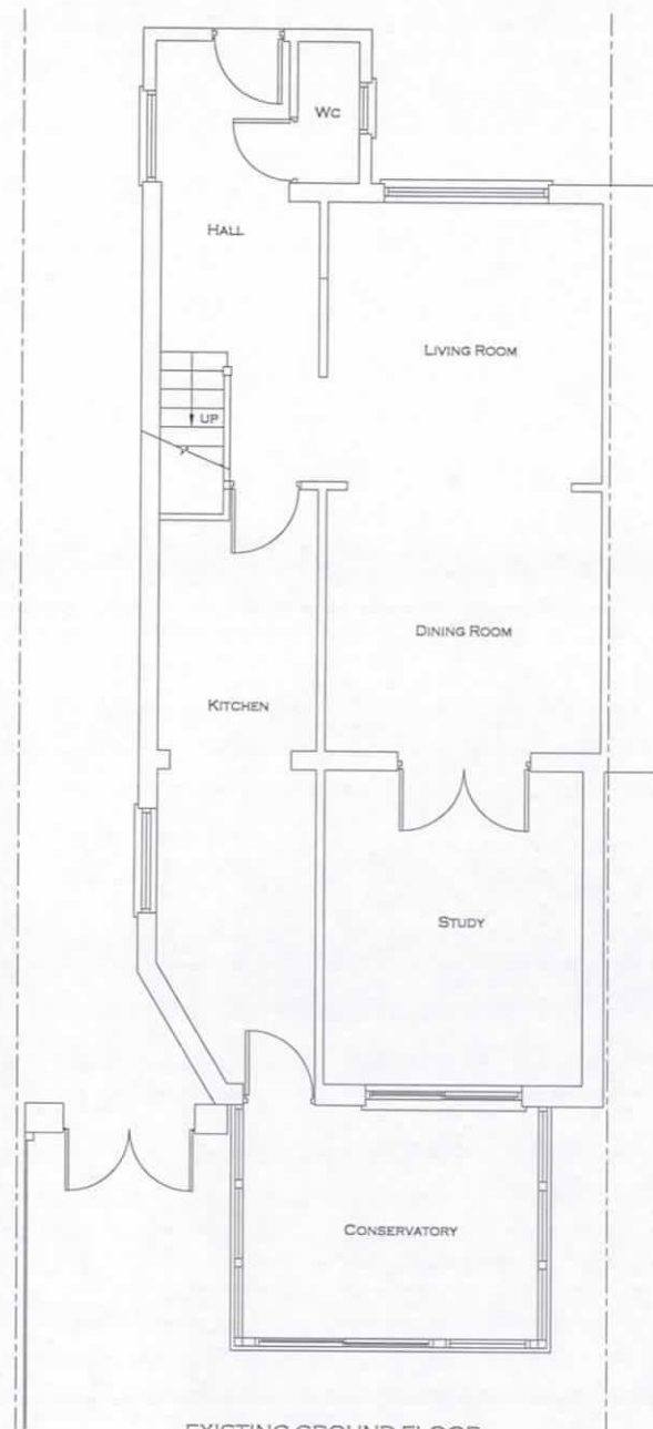
EXISTING GROUND FLOOR (No Change)
