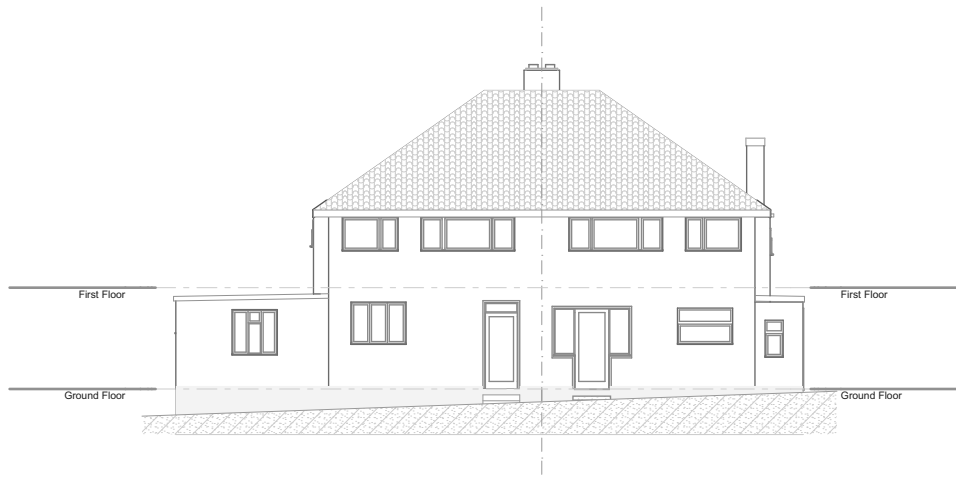
Existing Rear Elevation 1:200
