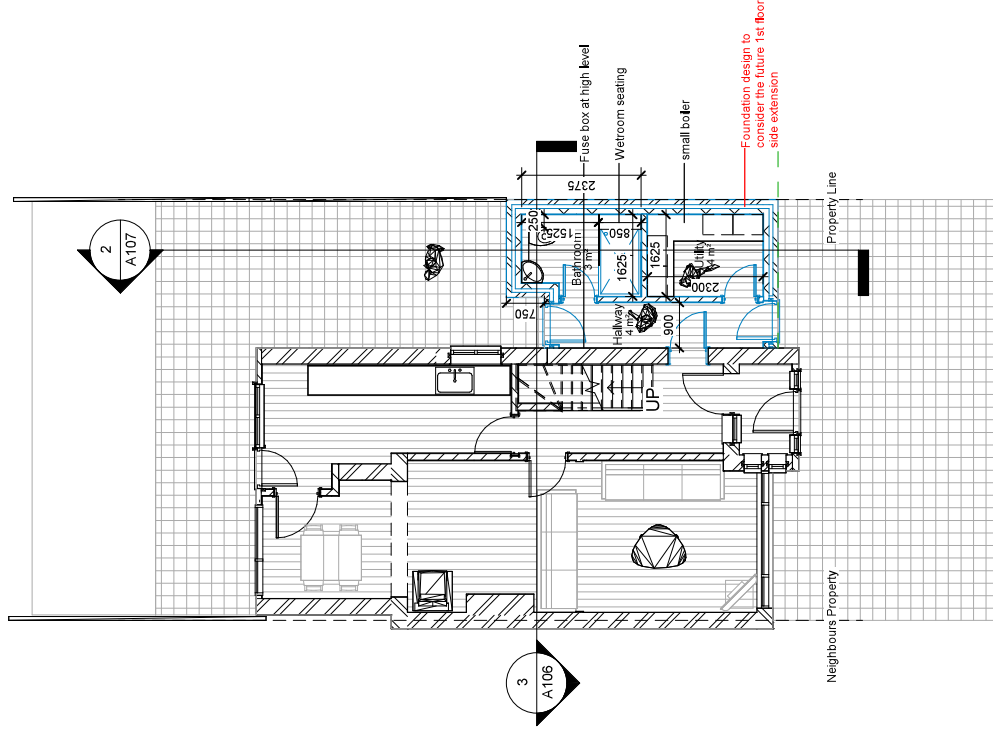
2 00 - Proposed 1 : 100
