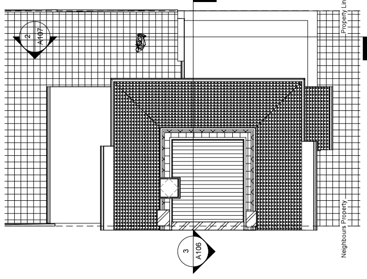
2 Loft - Proposed 1 : 100
