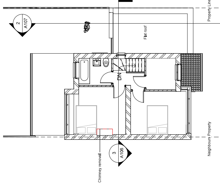
2 01-Proposed 1 : 100
