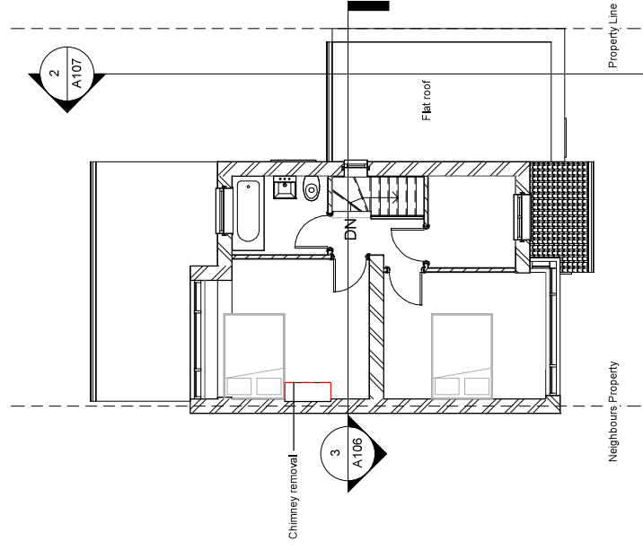
2 01- Proposed 1 : 100
