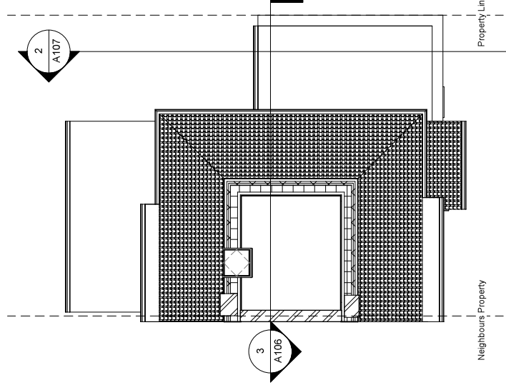
2 Loft - Proposed 1 : 100
