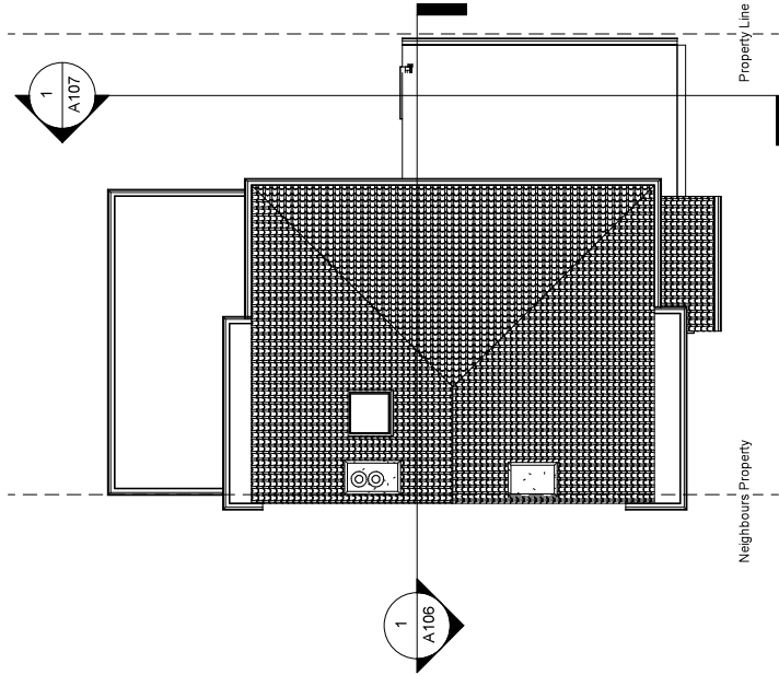
1 Roof - Existing
