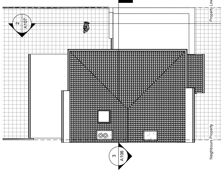
2 Roof - Proposed
