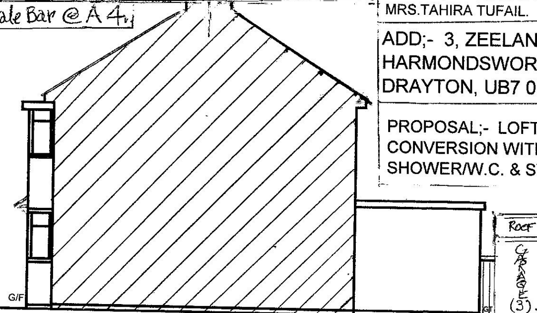
EXISTING SIDE VIEW OF (H/4) ELEVATION, (1:100).
