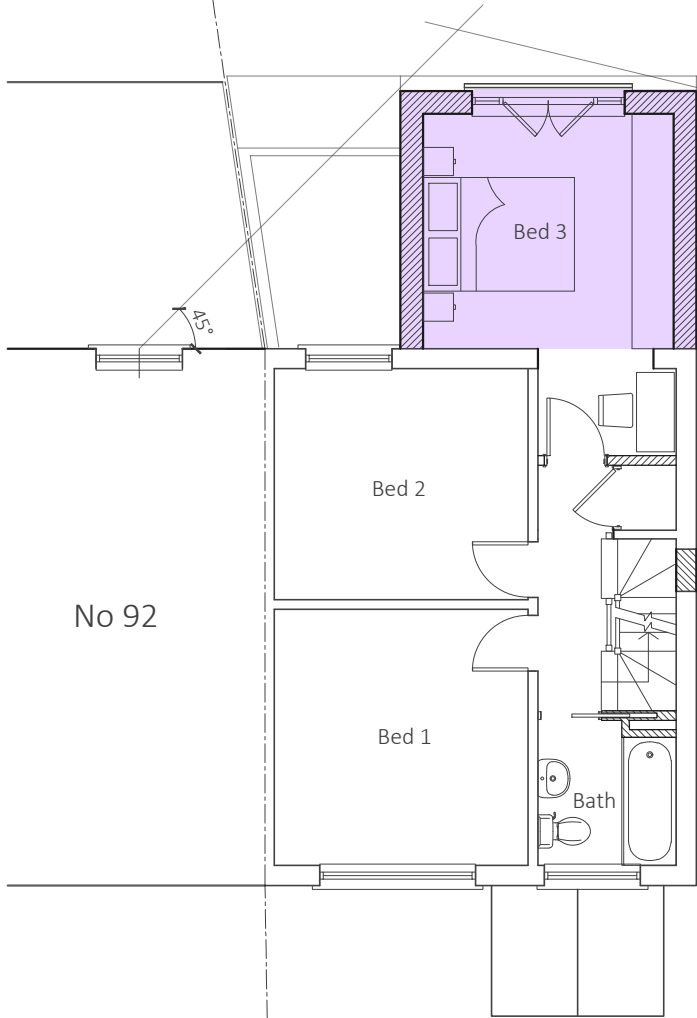
First Floor Plan, Retained
