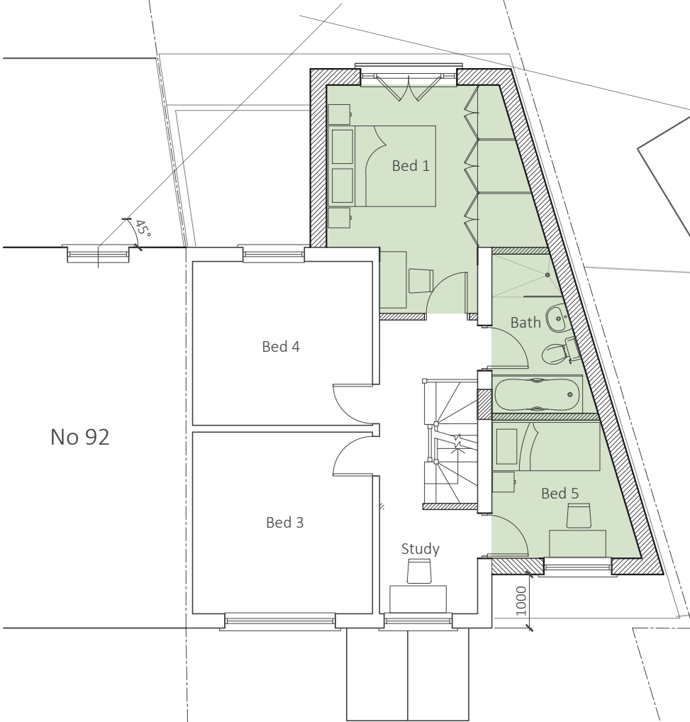
First Floor Plan, Retained
