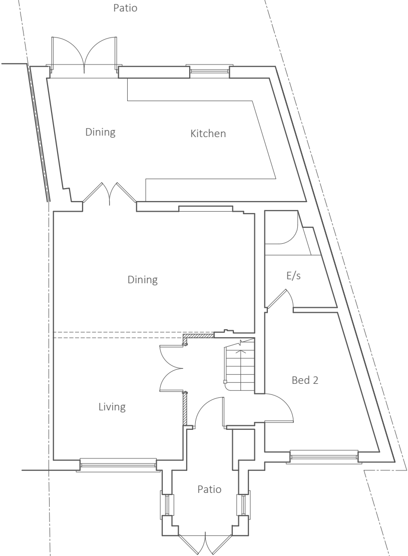
Ground Floor Plan, Proposed
