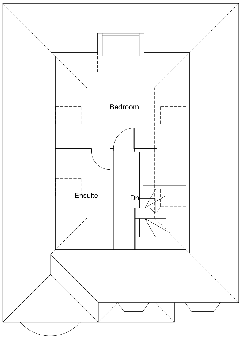
PROPOSED LOFT PLAN 1:100
