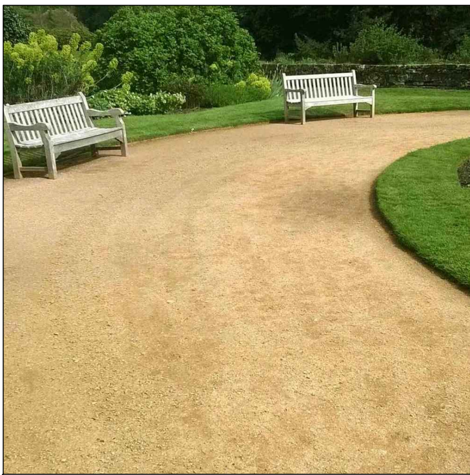
Bound gravel pathway New self binding gravel compacted surface, 40mm compacted thickness; on MOT type 1 sub base; material graded 12mm to dust; Breedon Aggregates Colour REF: Golden Amber: It is suitable for wheelchair use and meets the requirements under the Equality Act 2010; soft & natural appearance non trip, non slip surface
