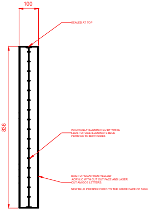
PROJECTING SIGN DETAIL SCALE 1:20
