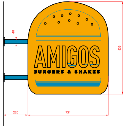
AMIGOS PROJECTED SIGN DETAILS
