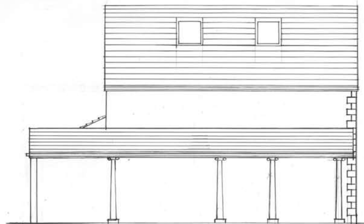
West Elevation
