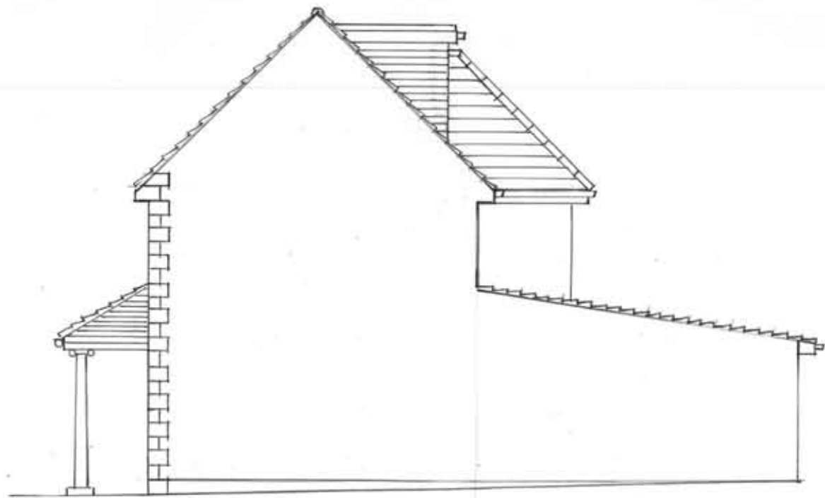
South Elevation
