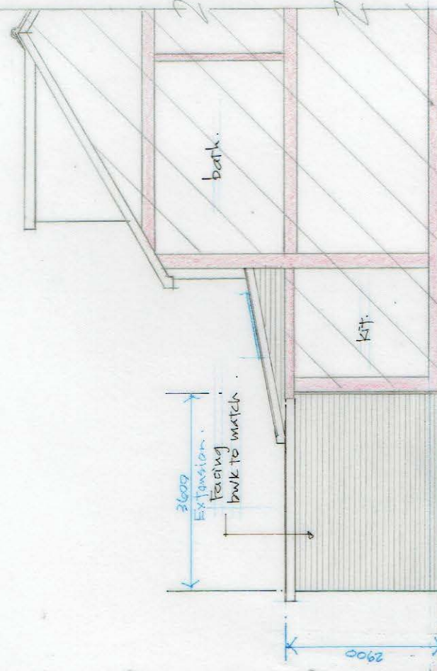
PROPOSED PART SECTIONAL SIDE ELEVATION.
