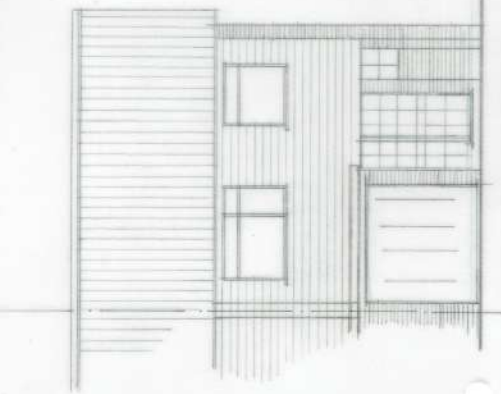
EXTG. FRONT ELEVATION.
