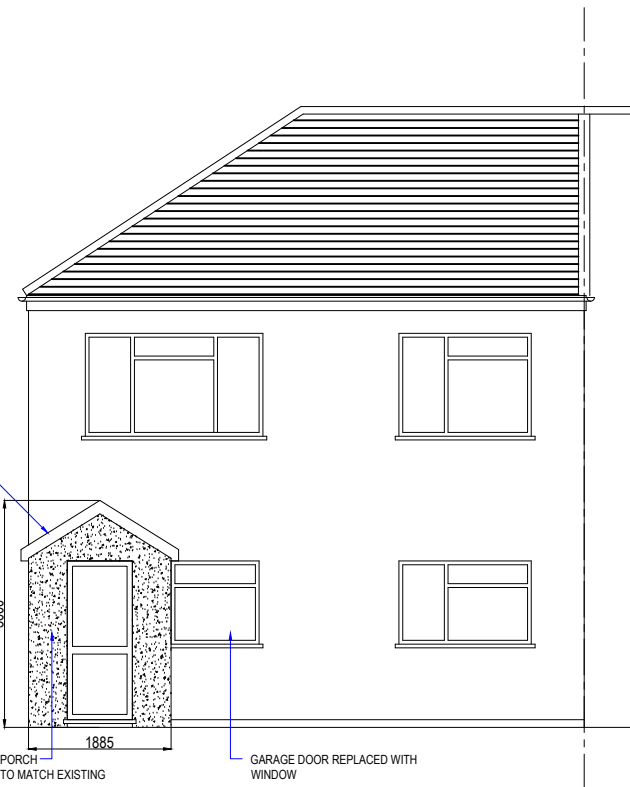
Front Elevation
