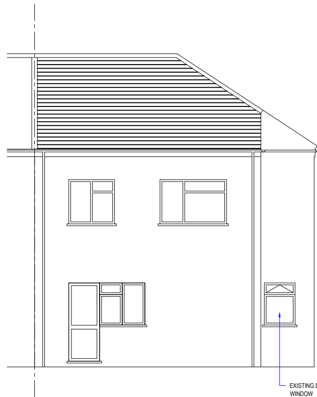
Rear Elevation
