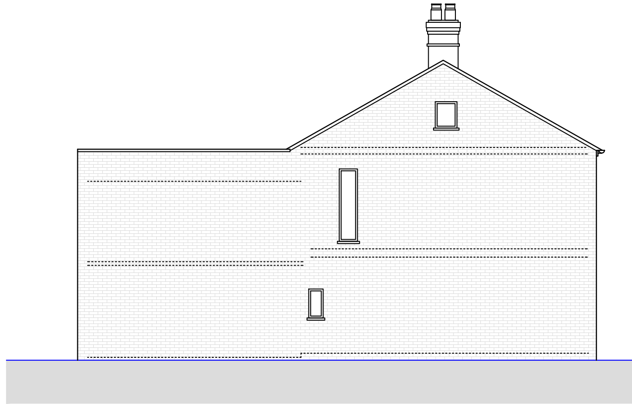
○ Side Elevation 1 1:100
