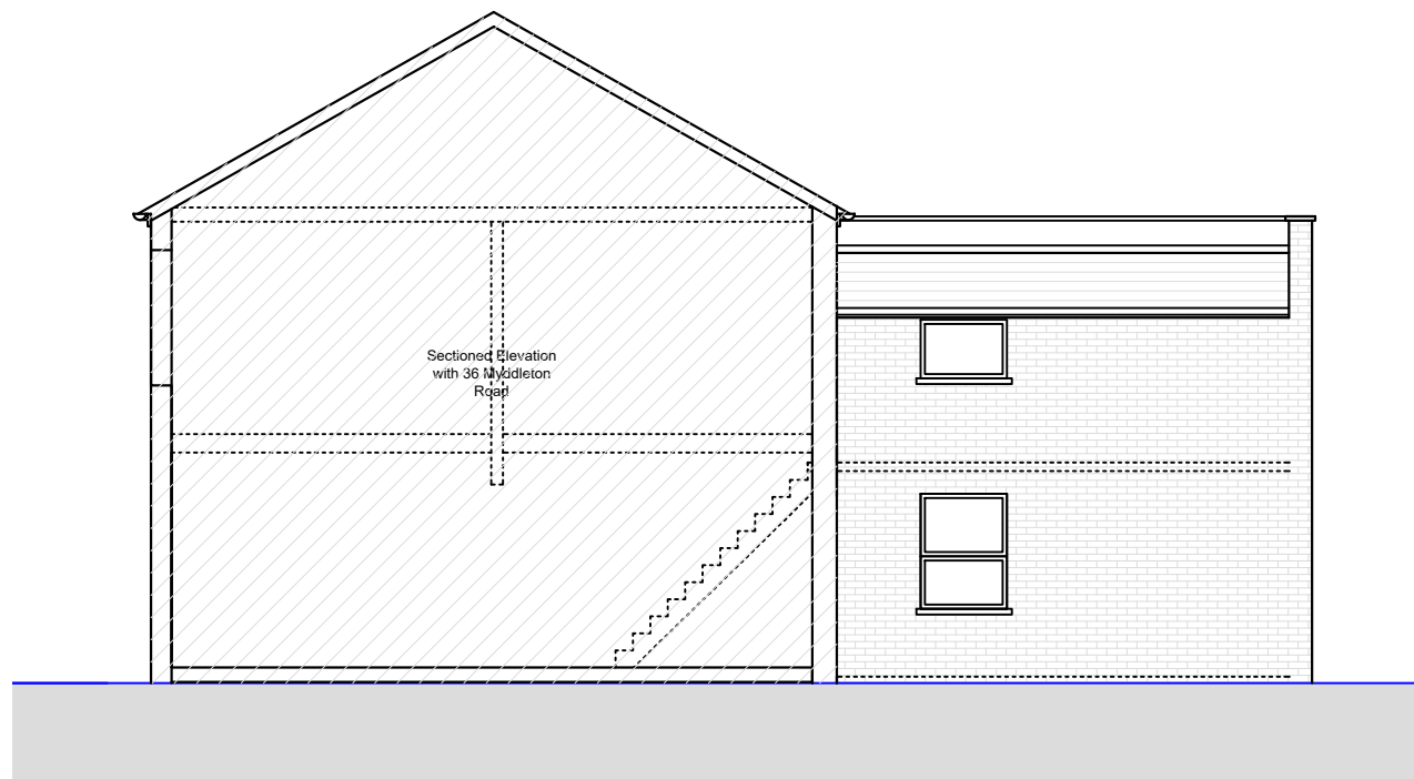
○ Sectioned Side Elevation 1:100
