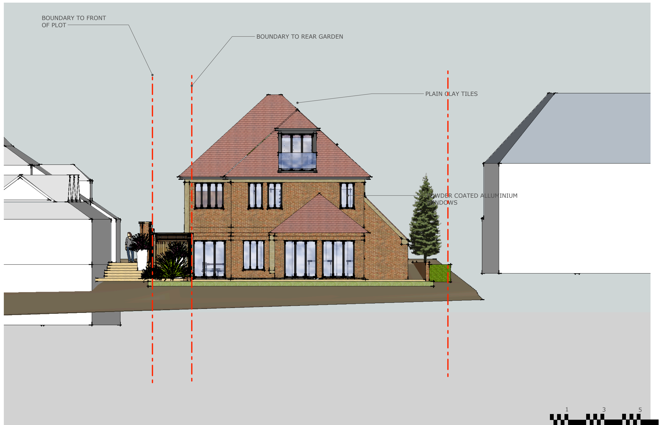
PROPOSED REAR ELEVATION- SOUTH EAST - 1.100
