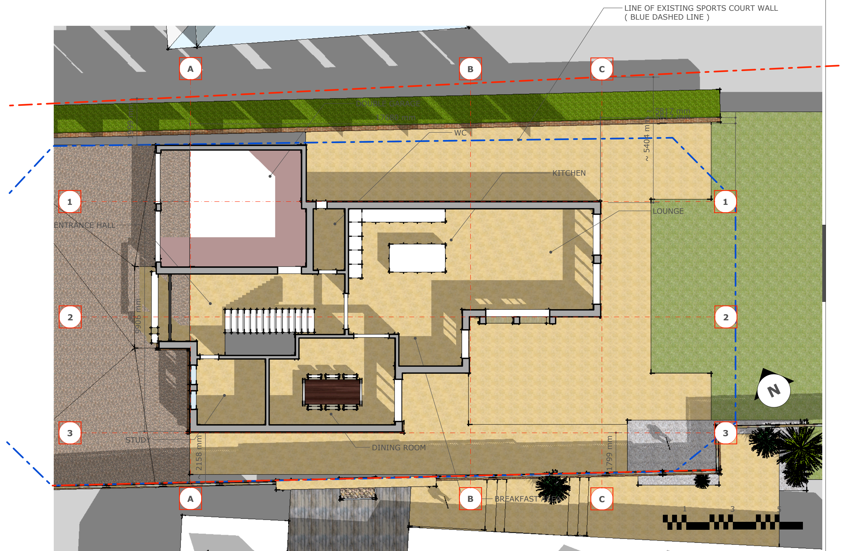
PROPOSED GROUND FLOOR LAYOUT - 1:100
