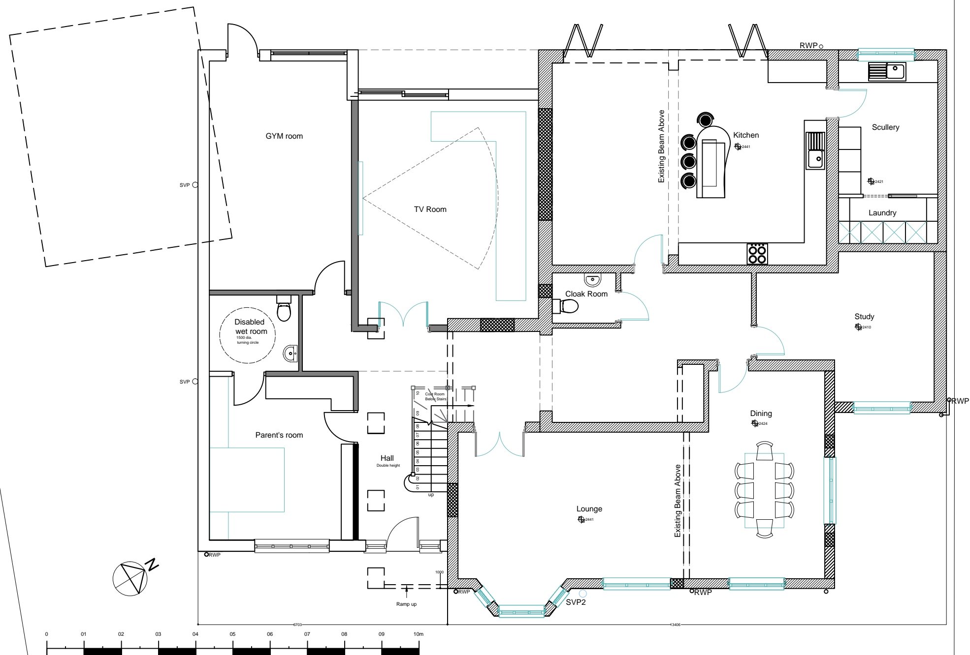
Proposed Ground Floor Plan (same as previously approved except for small internal changes)
