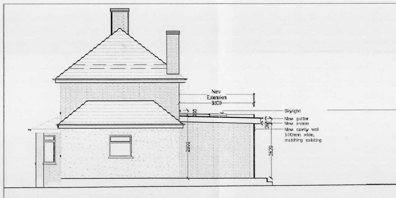
Elevation North - Proposed
