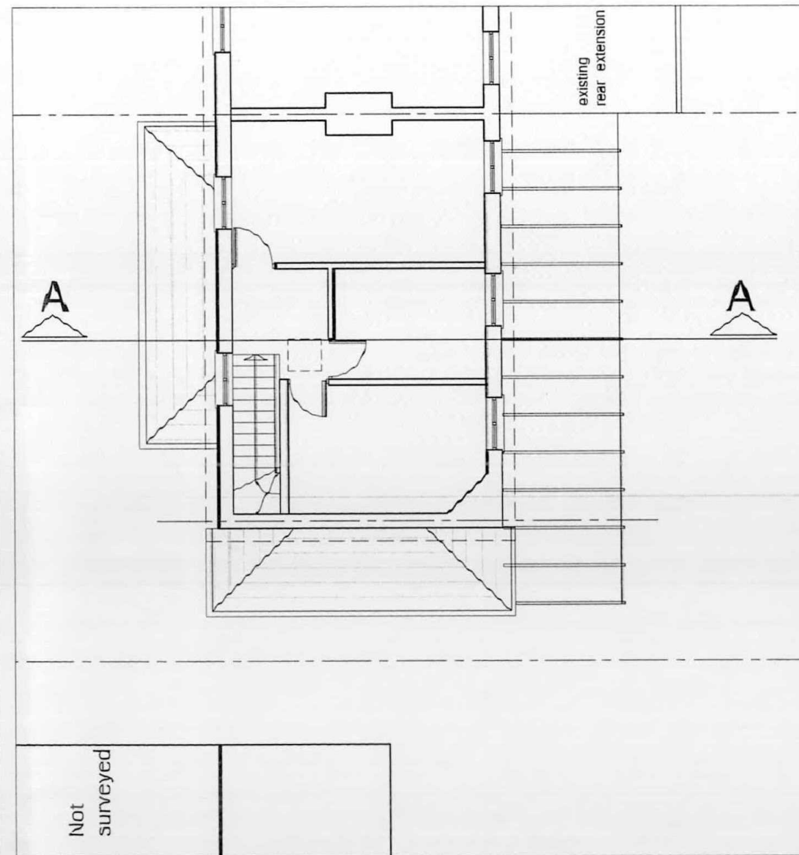
FF plan - Existing
