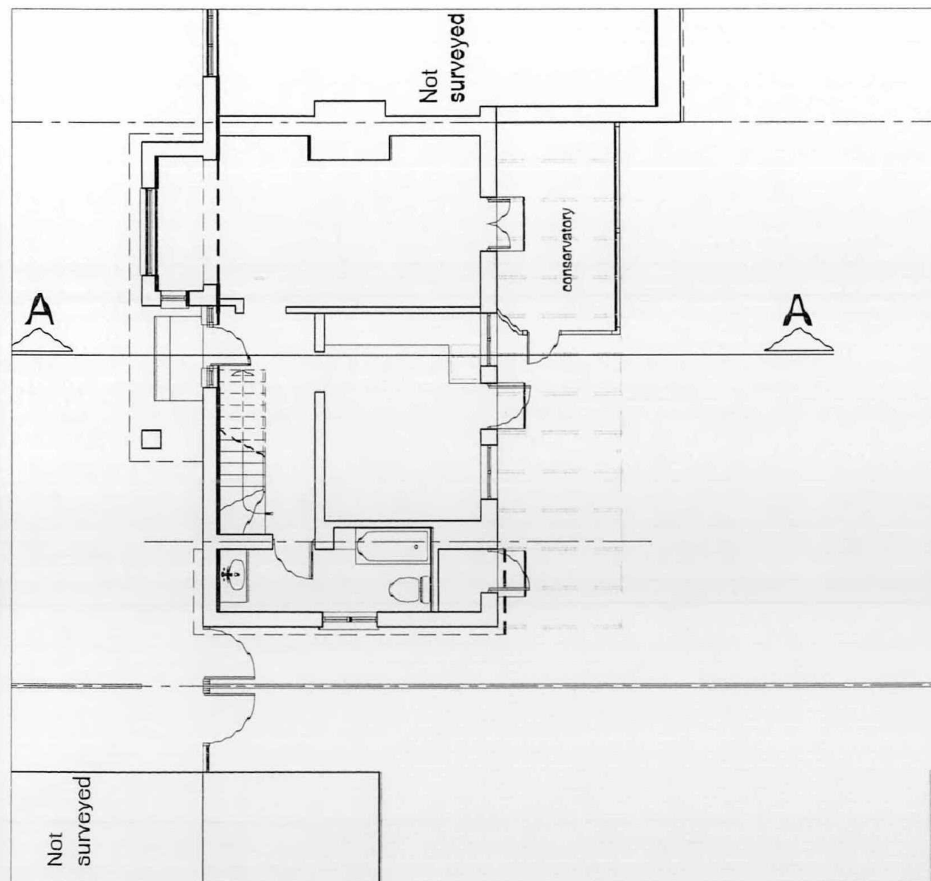
GF plan - Existing
