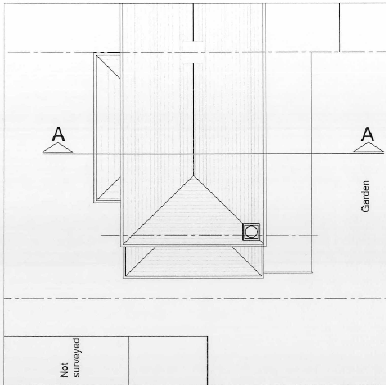
Roof plan - Existing
