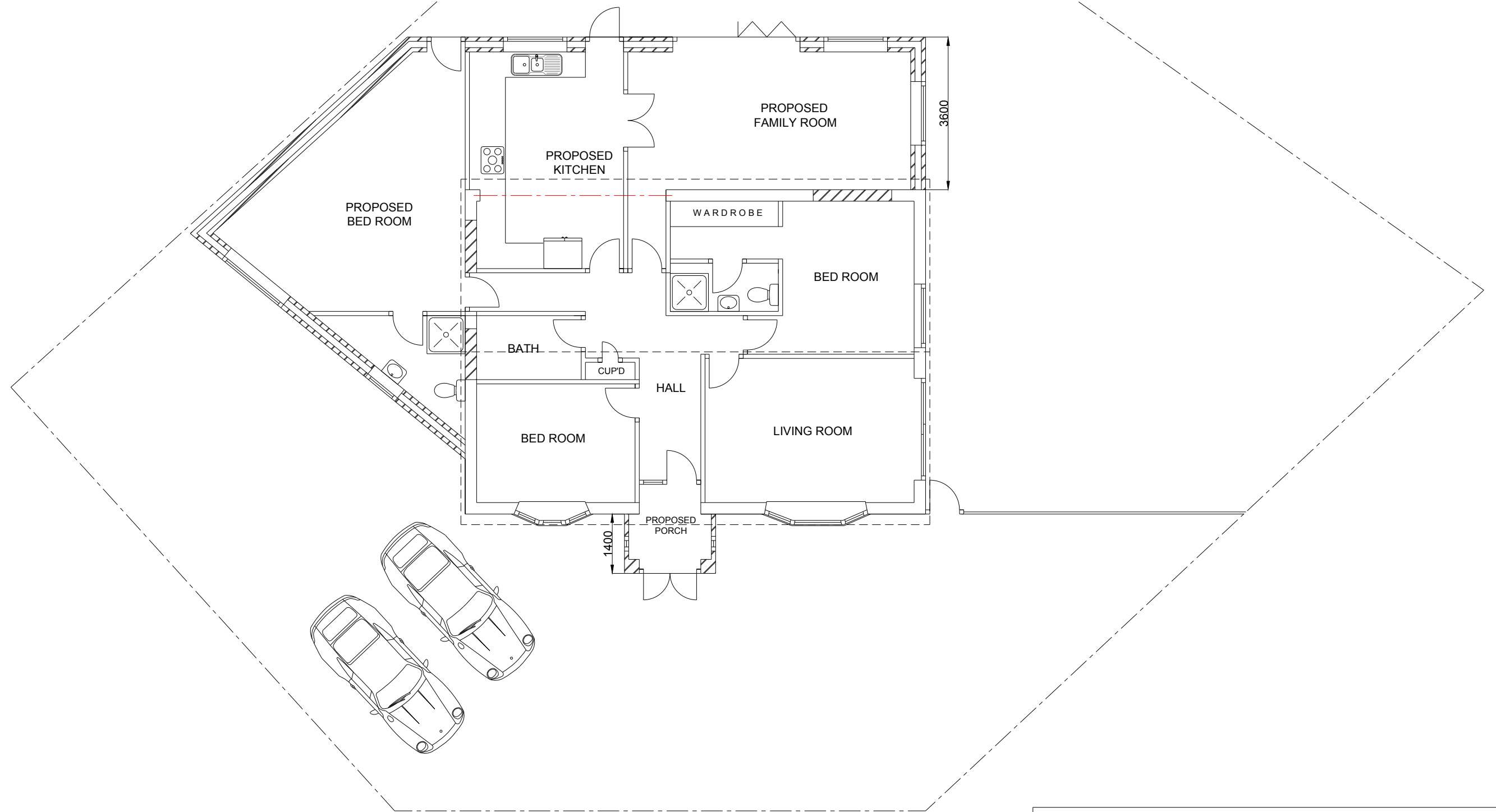
GROUND FLOOR PLAN PROPOSED
