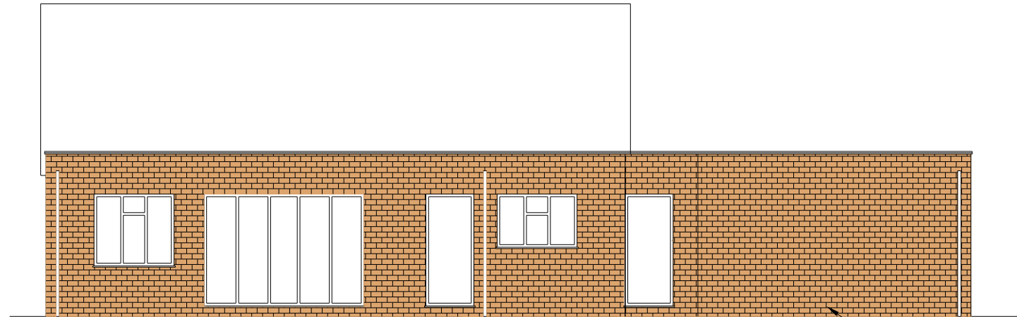
REAR ELEVATION PROPOSED
