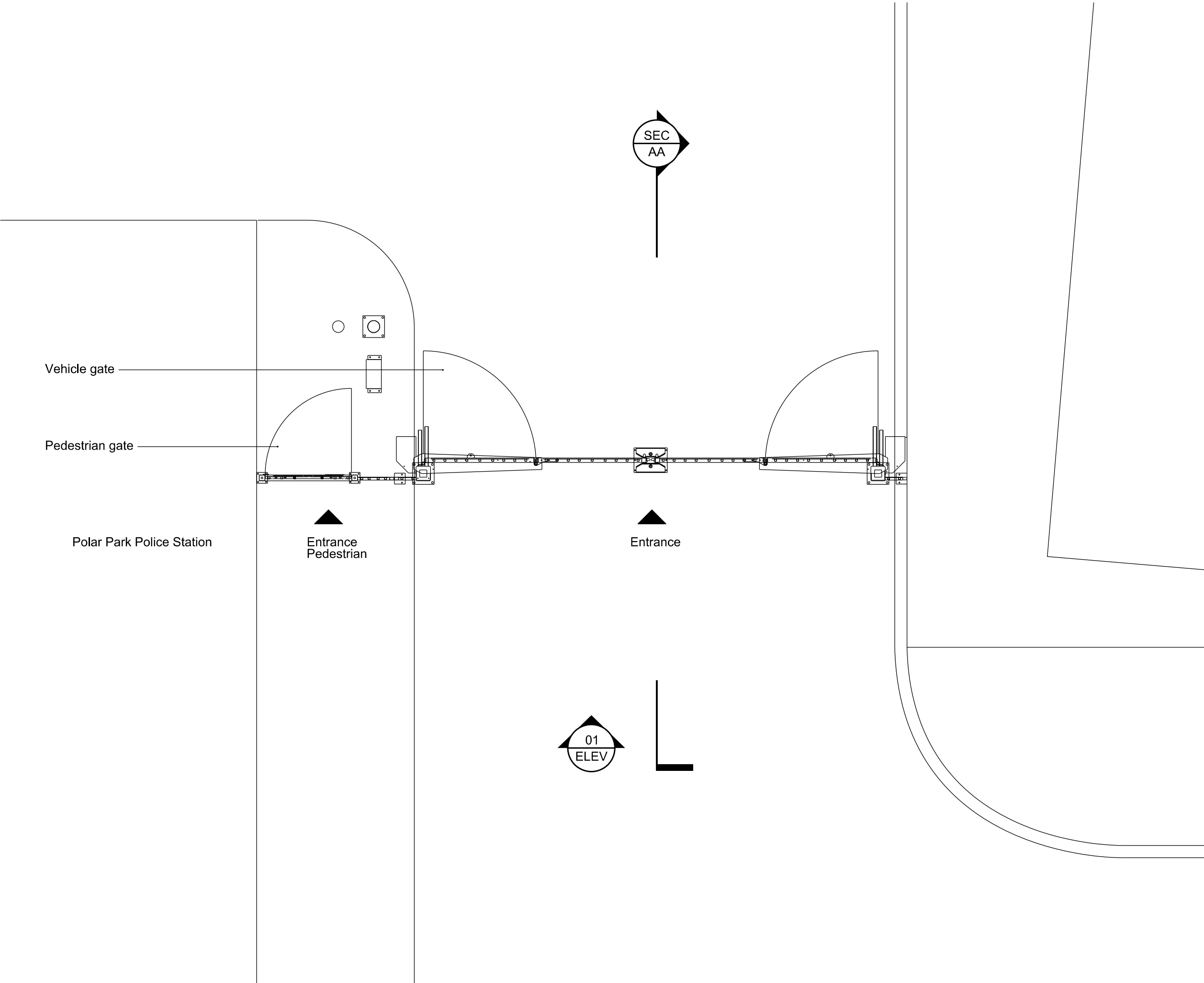
01 Plan - Existing 1:50
