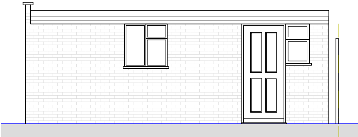
Side Elevation 1 1:50
