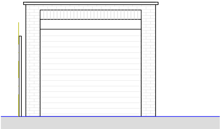
Front Elevation 1:50
