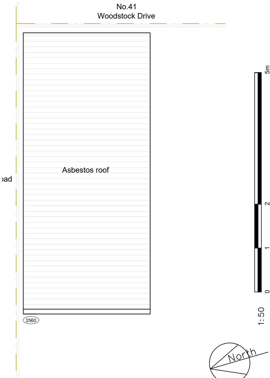
Roof Plan 1:50
