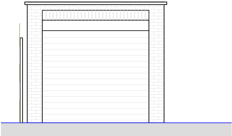
Rear Elevation 1:50
