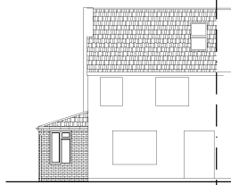
PROPOSED FRONT ELEVATION
