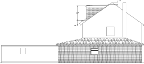
PROPOSED SIDE ELEVATION
