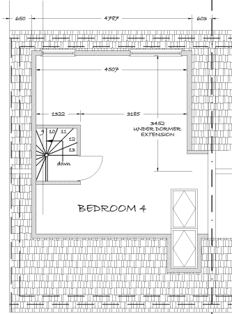
PROPOSED ROOF AND SECOND FLOOR PLAN
