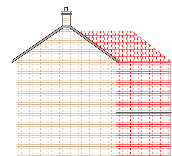
AMENDMENT PROPOSED SIDE ELEVATION
