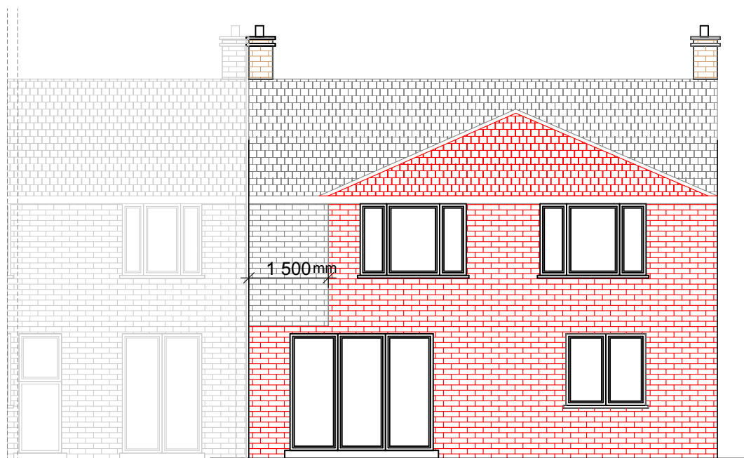
AMENDMENT PROPOSED REAR ELEVATION
