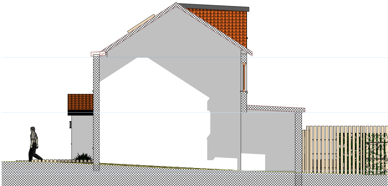
SOUTH ELEVATION
