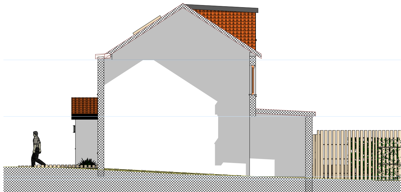
SOUTH ELEVATION
