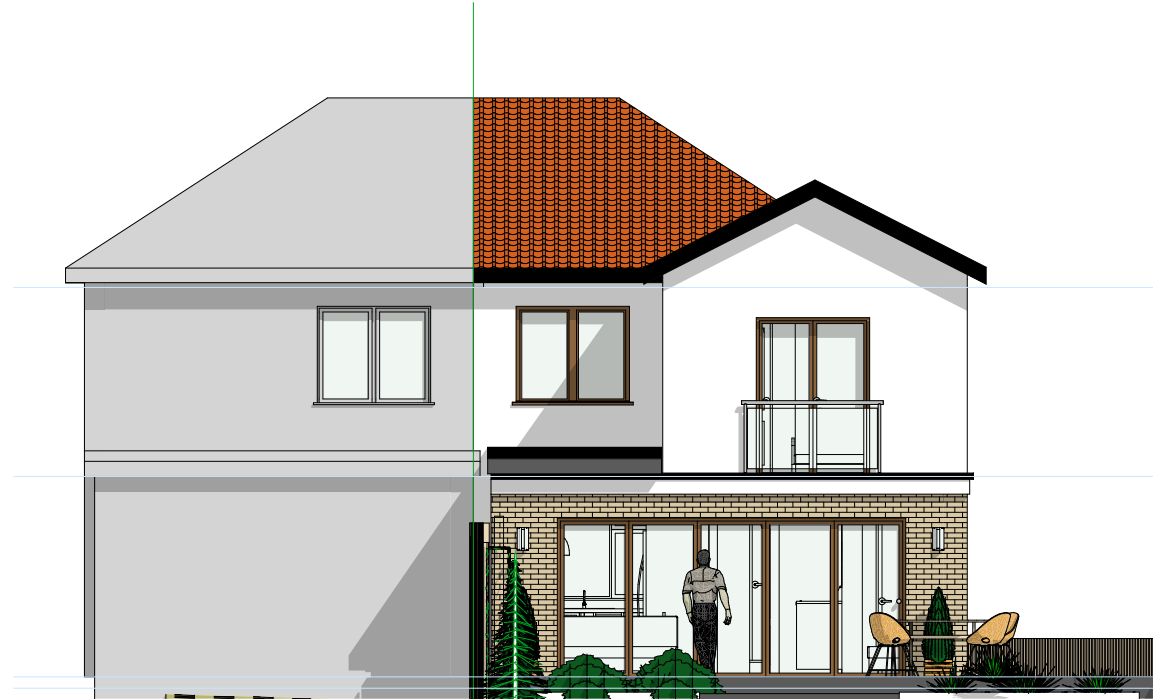
EAST REAR ELEVATION
