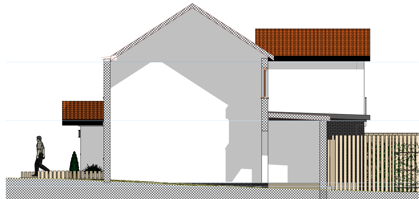
SOUTH ELEVATION
