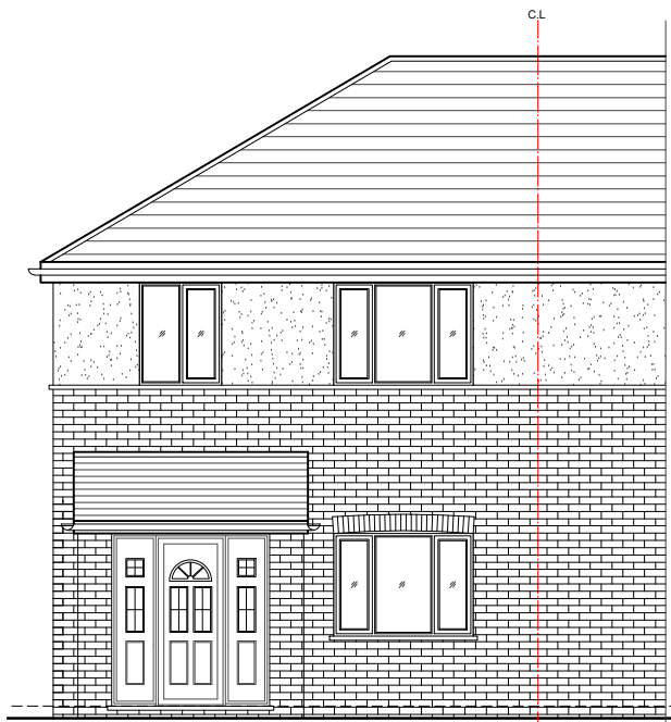
04 - FRONT ELEVATION
