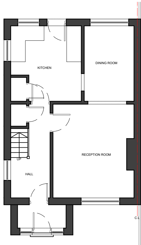
01 - GROUND FLOOR PLAN
