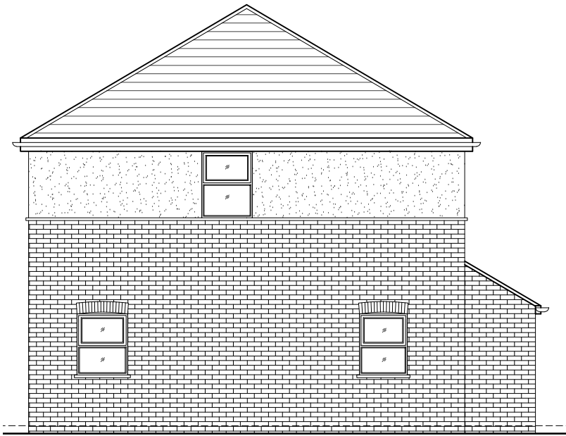
05 - SIDE ELEVATION
