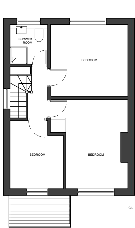
02 - FIRST FLOOR PLAN
