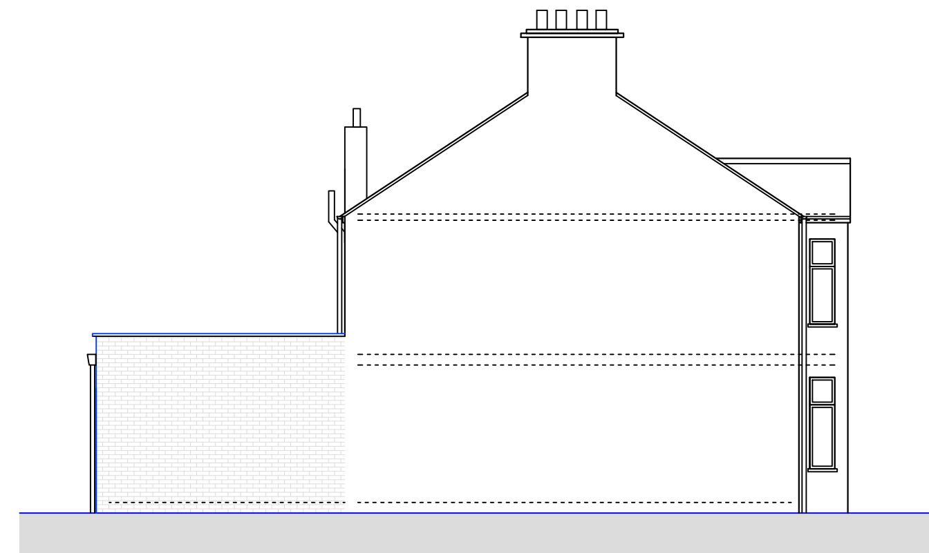
○ Side Elevation 2 1 : 1 0 0
