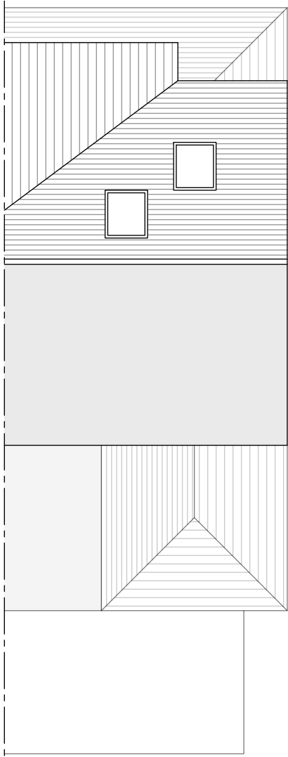
ROOF PLAN
