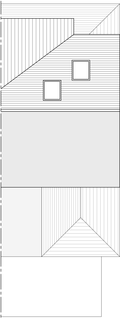
ROOF PLAN
