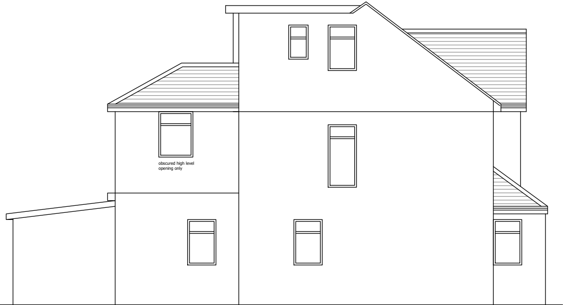
SIDE ELEVATION
