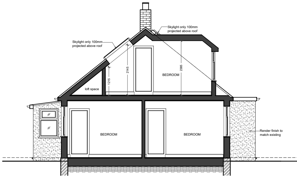
05 - PROPOSED SECTION AA
