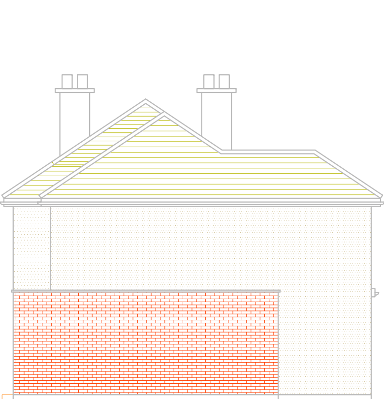
PROPOSED SIDE ELEVATION-1
