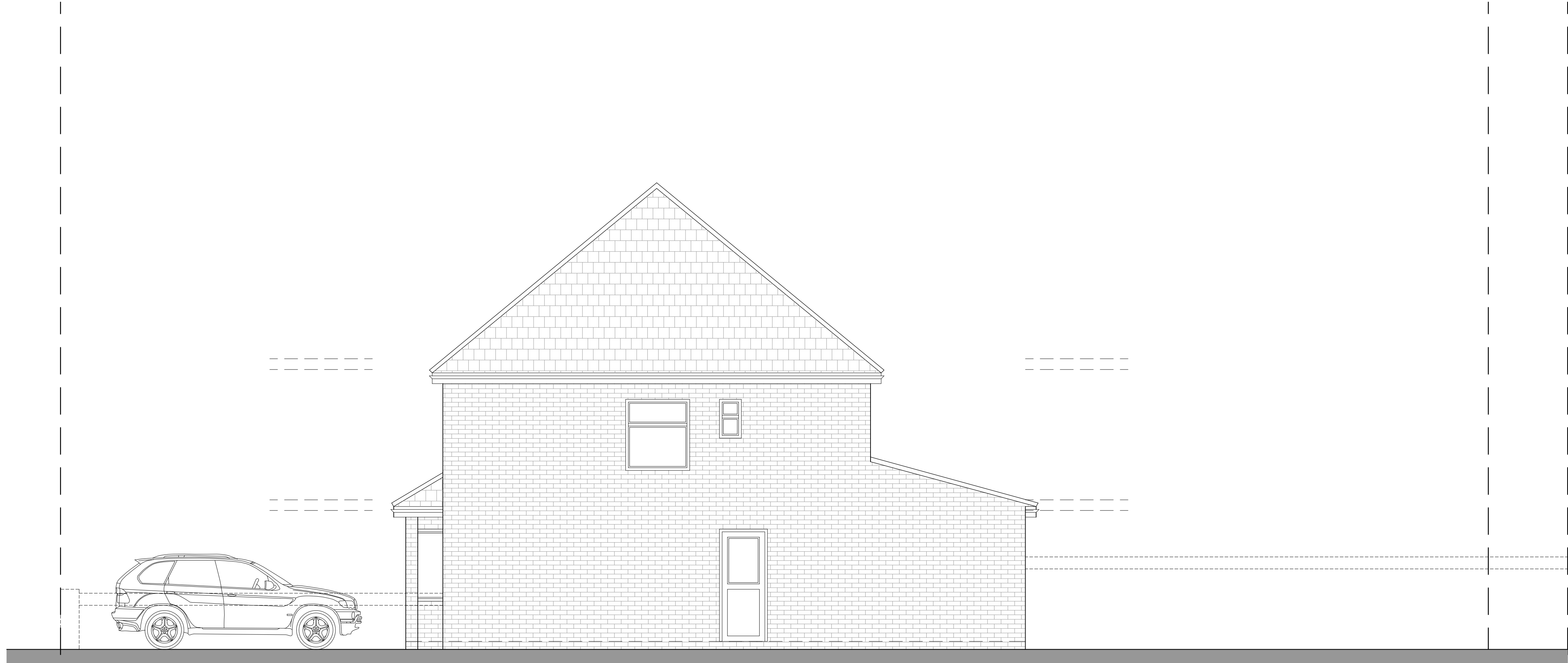
Proposed Side Elevation Scale 1:50
