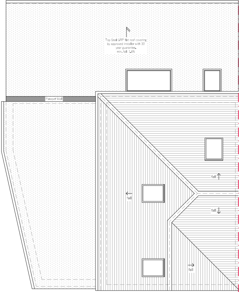
ROOF PLAN
