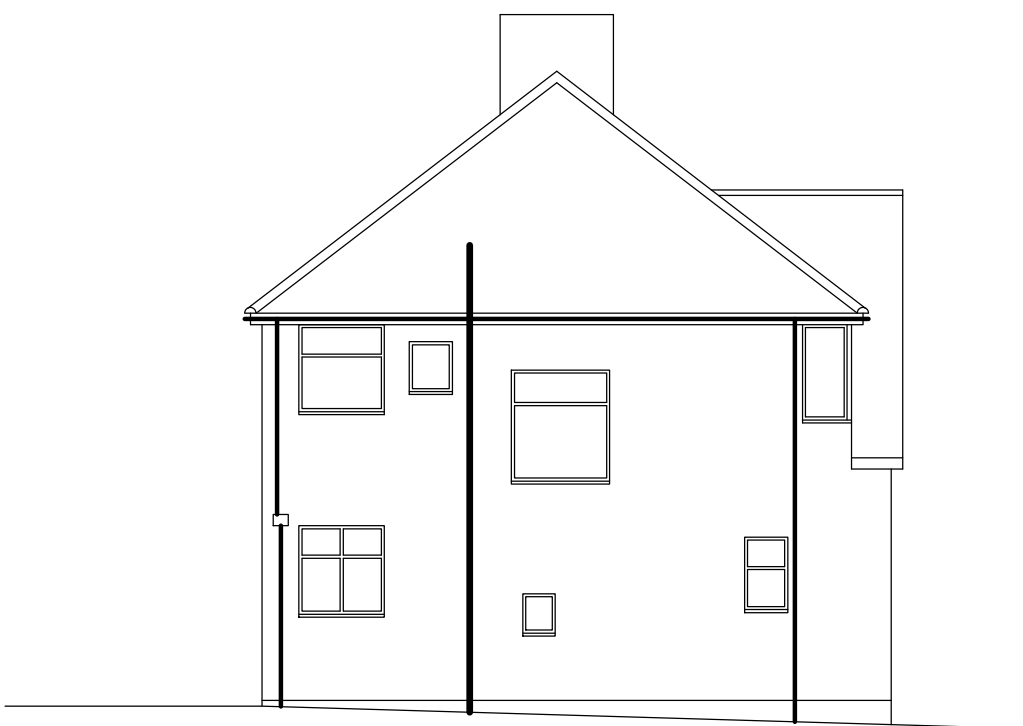
LEFT ELEVATION (1:100)
