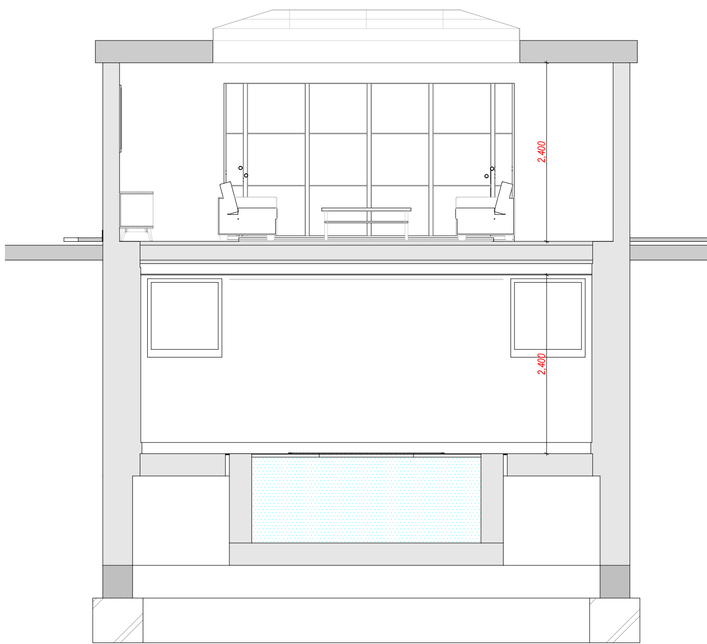
S-08 Building Section 1:50
