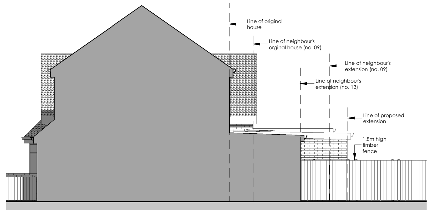
2 Proposed North Side Elevation 2423-A-302 1 : 100
