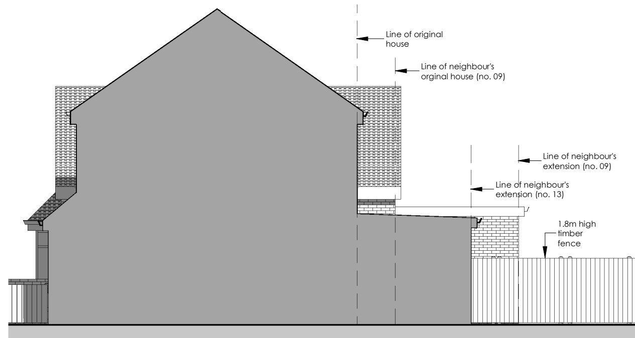
1 Existing North Side Elevation 2423-A-302 1 : 100
