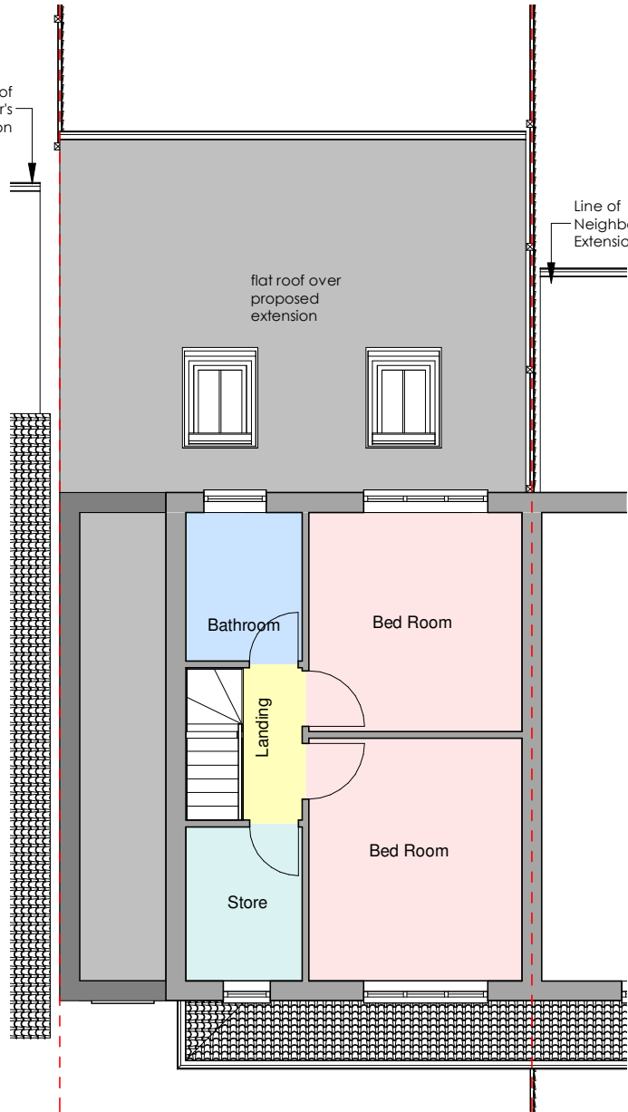
2 Proposed First Floor 2423-A-301 1 : 100
