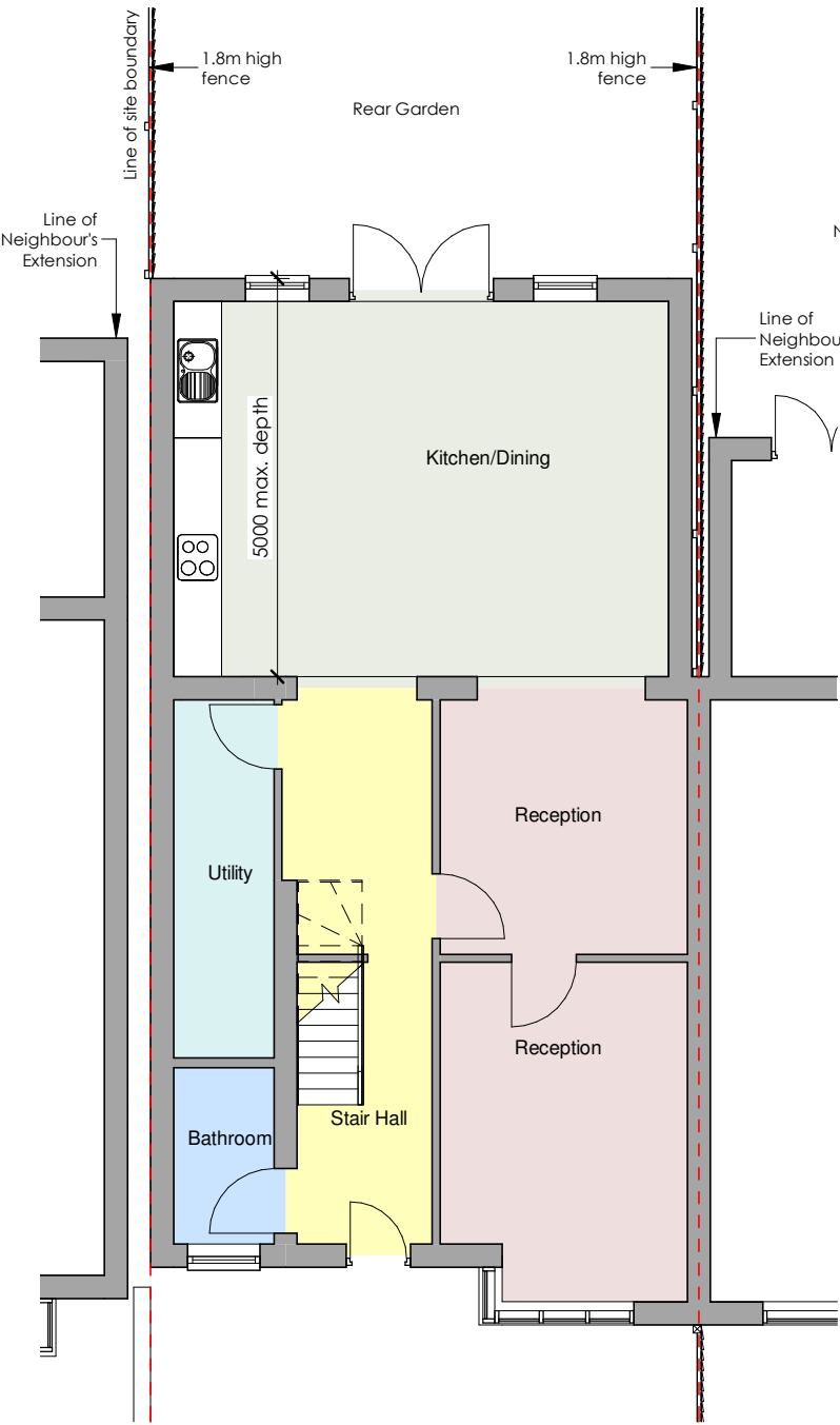
1 Proposed Ground Floor 2423-A-301 1 : 100
