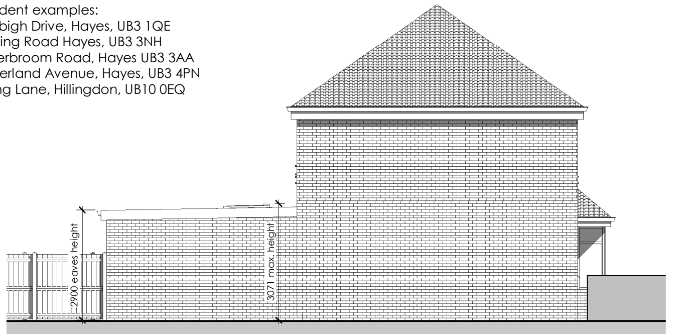
5 Proposed Side Elevation 2423-A-301 1 : 100
