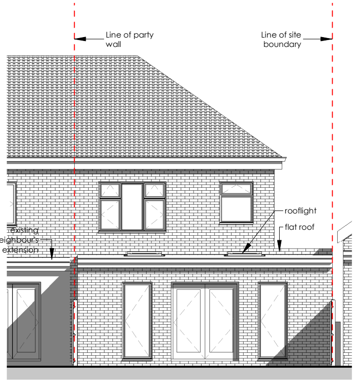
4 Proposed Rear Elevation 2423-A-301 1 : 100
